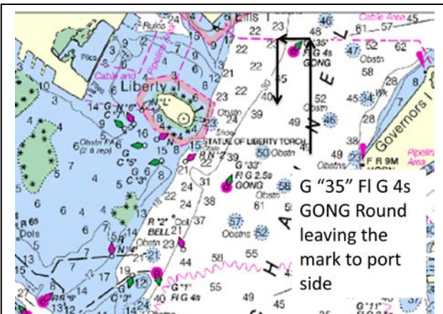
Fig A3: Round (in either direction) Channel Marker G "35" FI G 4s GONG.
